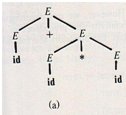
Two parse trees for id + id * id
