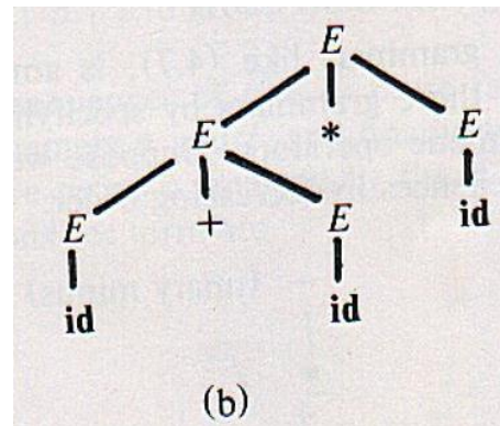
Two parse trees for id + id * id
