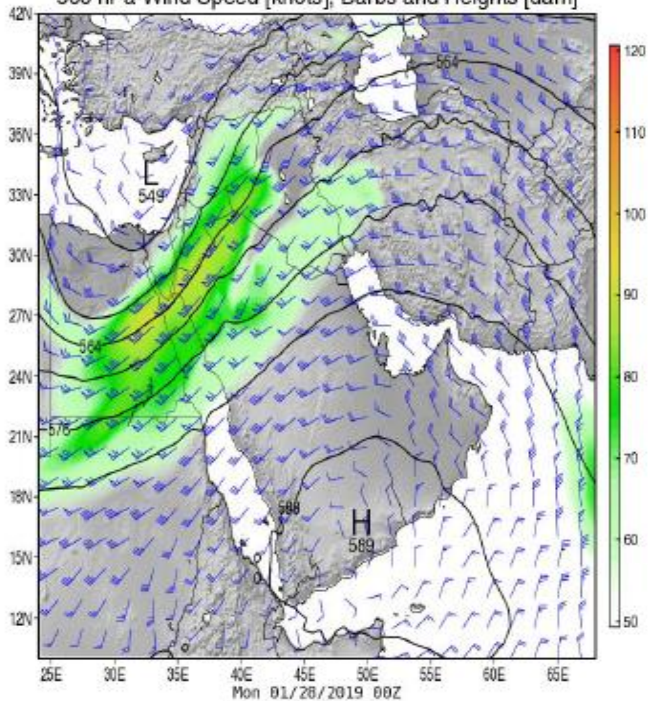
500 hPa Wind Speed [knots], Barbs and Heights [dam]
