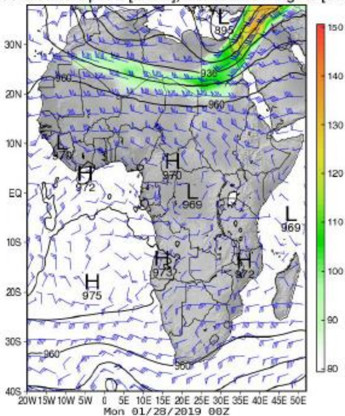
300 hPa Wind Speed [knots], Barbs and Heights [dam]
