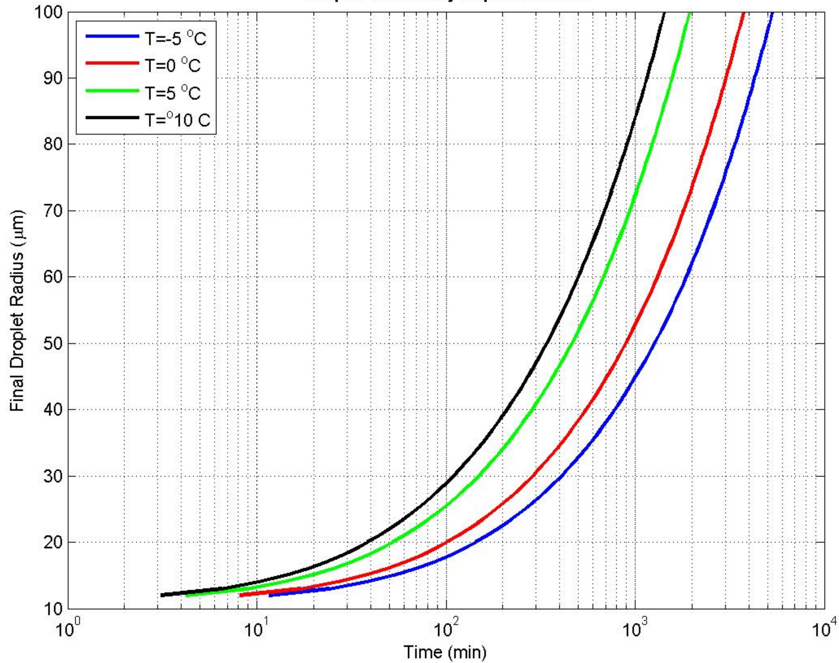
Droplet Growth by Vapor Diffusion
