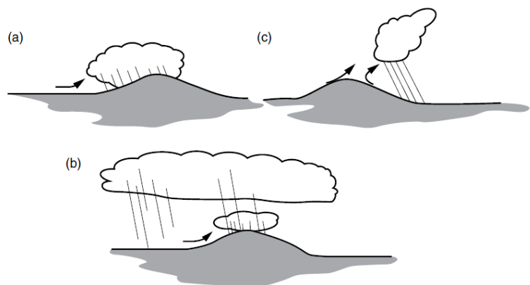
Figure (3.6) Mechanisms of orographic rain generation
