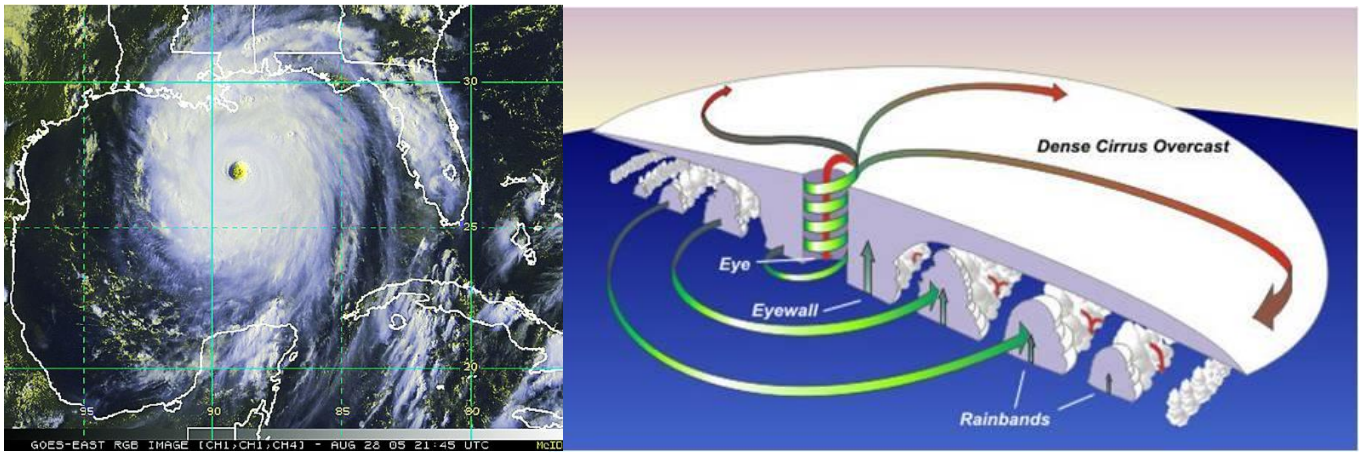
Figure (3.5) (Left) Hurricane Katrina, 28 /8/ 2005; category 5, highest winds 175 mph ( 280 \text{ km h}^{-1} ), lowest pressure 902 mbar (hPa). (Right) typical vertical structure of tropical depression (hurricane).
