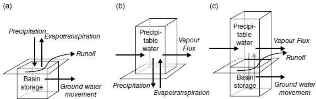
Figure 1.3 Illustrating (a) terrestrial water balance, (b) atmospheric water balance and (c) combined atmospheric-terrestrial water balance
