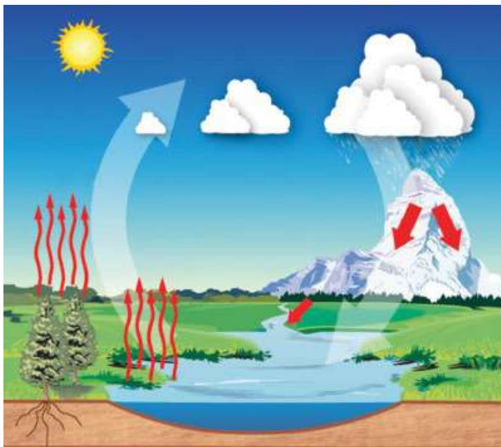
Figure 1.1 Simplified representation of the hydrological cycle
