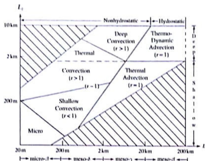
Fig. 1.2 Schematic of flow regimes under unstable stability conditions, where hatched zones indicate nonphysical flow regimes, the dotted line indicates merging of thermo-dynamic advection with macroscale, r represents scaled ratio of buoyancy and vertical pressure gradient forced perturbations, and the dashed line represents division of thermal convection into its deep and shallow regimes. (Adapted after Thunis and Bornstein 1996.)
