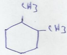
1,2-dimethylcyclohexane
