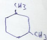
1,3-dimethylcyclohexane
