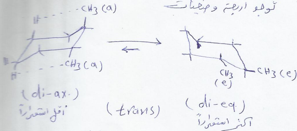
1,2-dimethylcyclohexane
