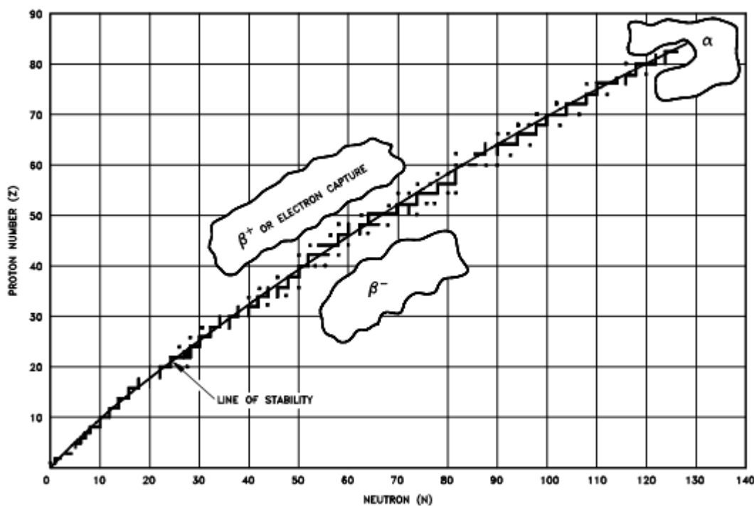
Figure (3-2): Types of Radioactive Decay Relative to the Line of Stability.
