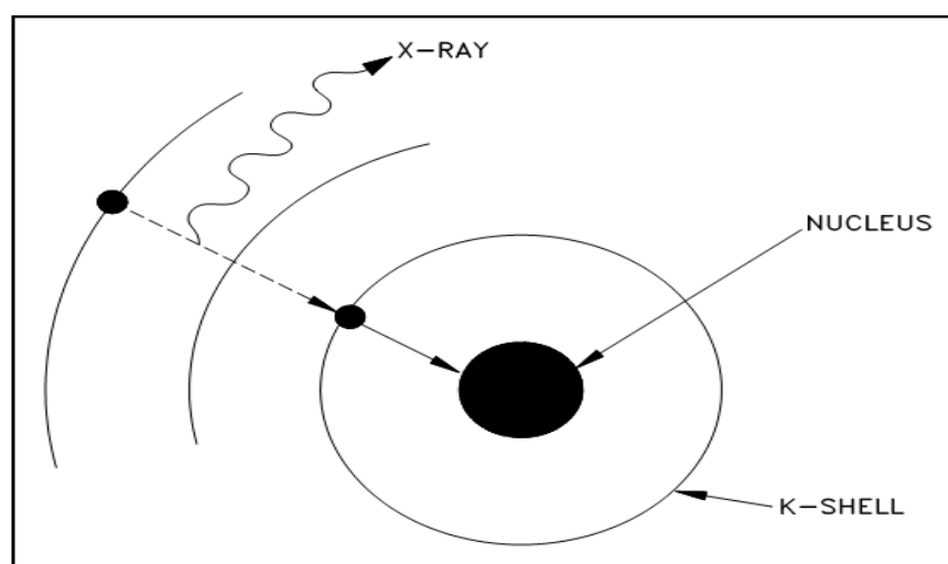
Figure (3-1): orbital electron capture.
