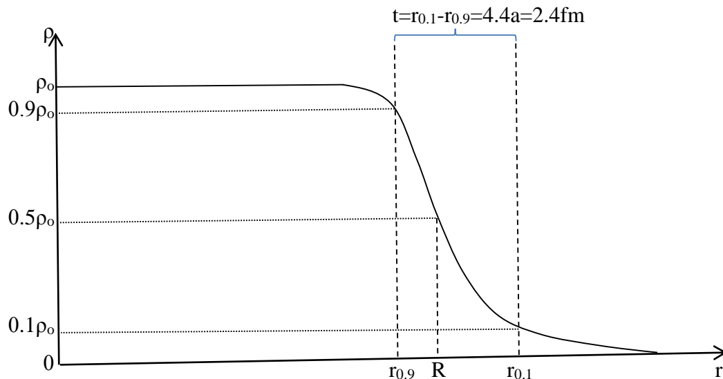
Figure (1-2): plot of nuclear density equation \rho(r) Vs. r , the meaning of \rho_o , R and a are illustrated.
