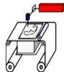
Laminated-object manufacturing
