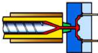
Injection molding
