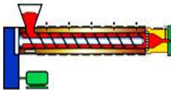
Extrusion
