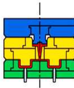
Transfer molding
