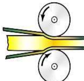
Cold welding
