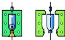
Blow molding
