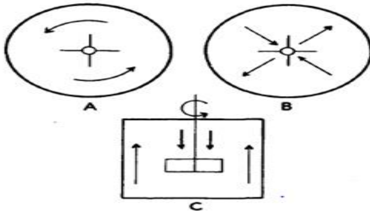
FIG. 1-2. A and B, Diagrammatic representation of cylindric tanks in which tangential and radial flow occur, respectively. C, Side view of a similar tank in which axial flow occurs. These diagrams represent systems in which only one type of flow occurs, in contrast to the usual situation in which two or more of these flow patterns occur simultaneously.
